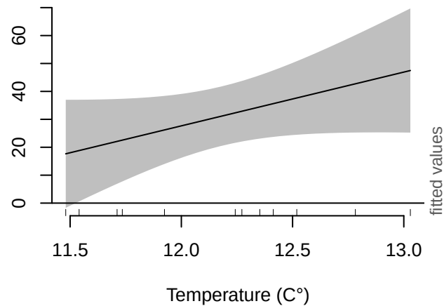
Grey Seal
