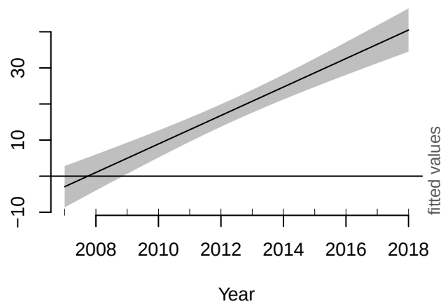
Harbor Seal
