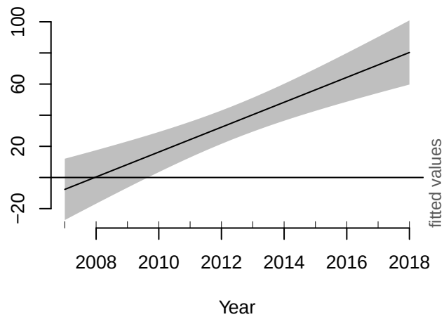
Grey Seal
